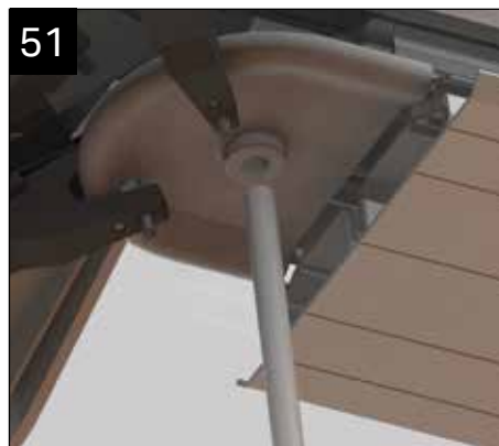
51 Insert the nylon threaded bar into the bottom of the spider.
